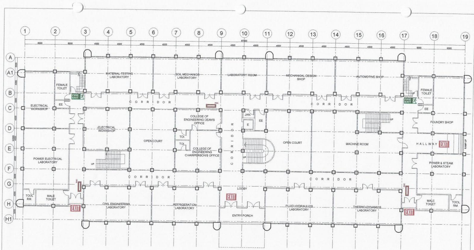
1 A-1 GROUND FLOOR PLAN SCALE 1:300MTS
