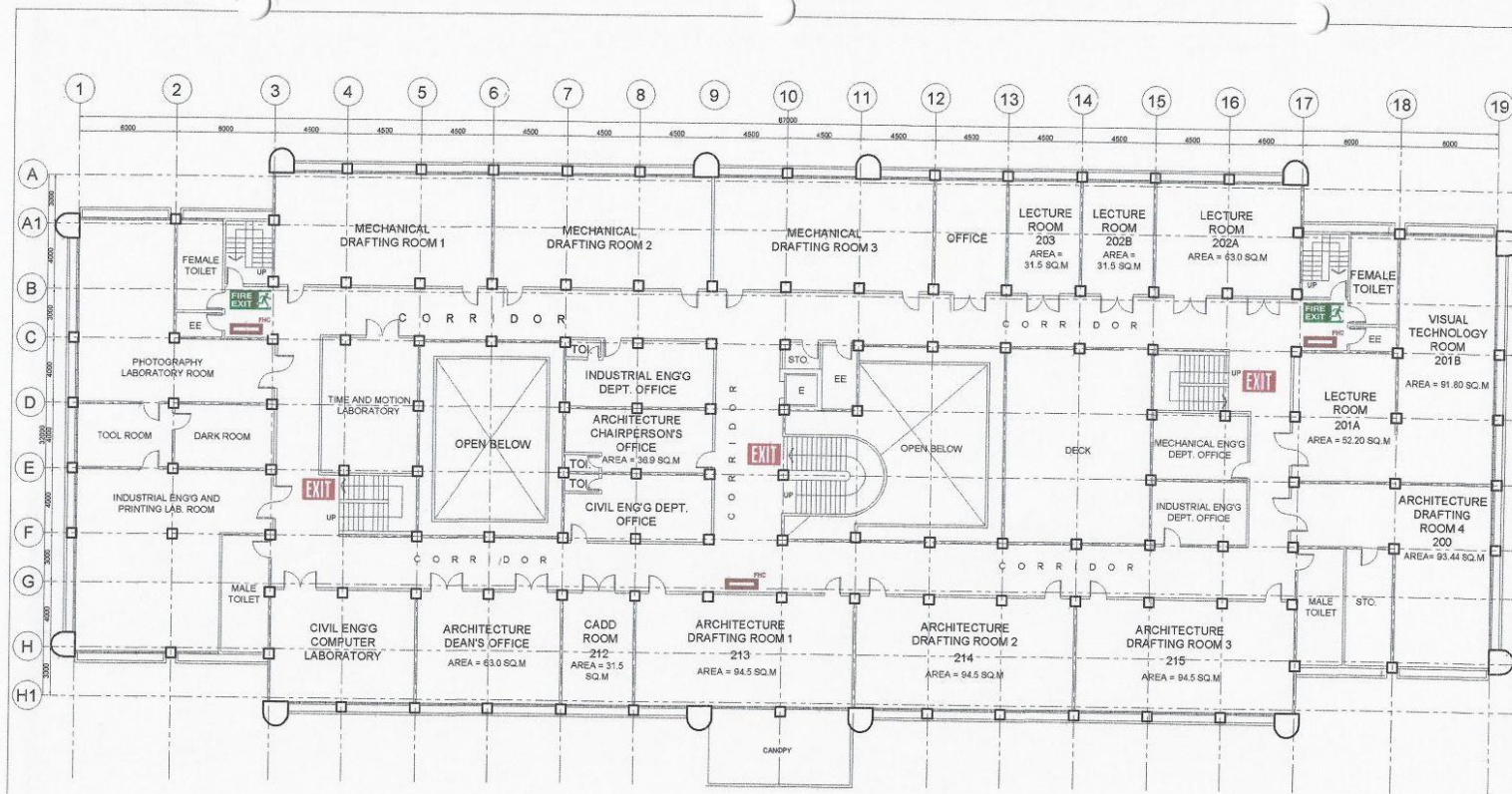
1 SECOND FLOOR PLAN SCALE 1:300M TS
