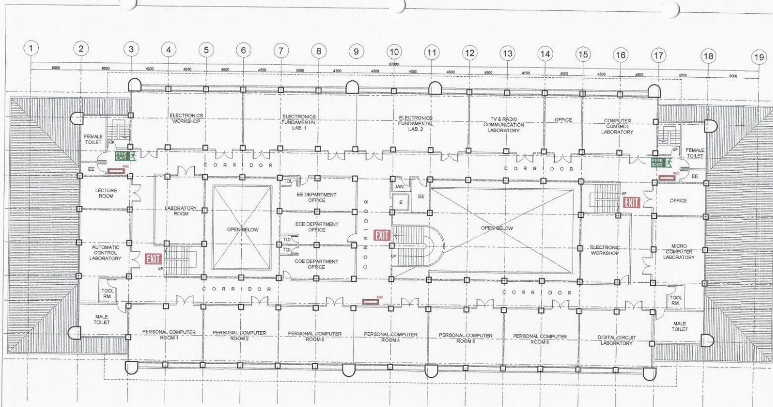
1 A-3 THIRD FLOOR PLAN SCALE 1:300MTS
